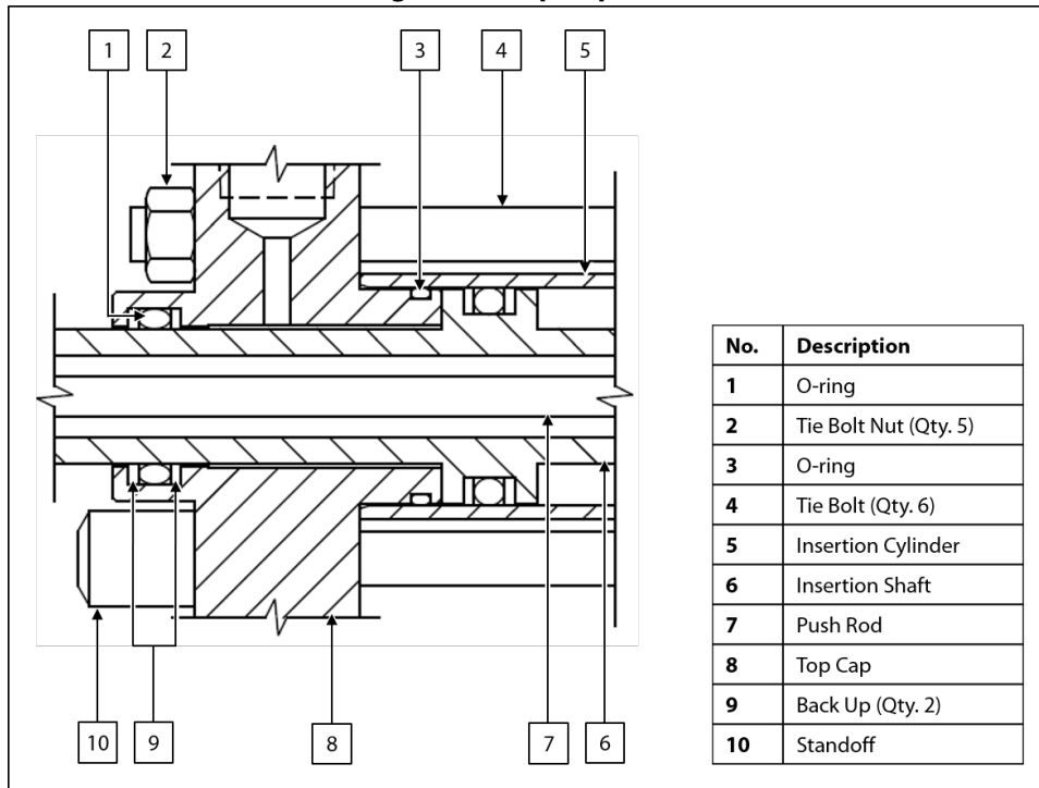
Figure 11: Top Cap Detail
