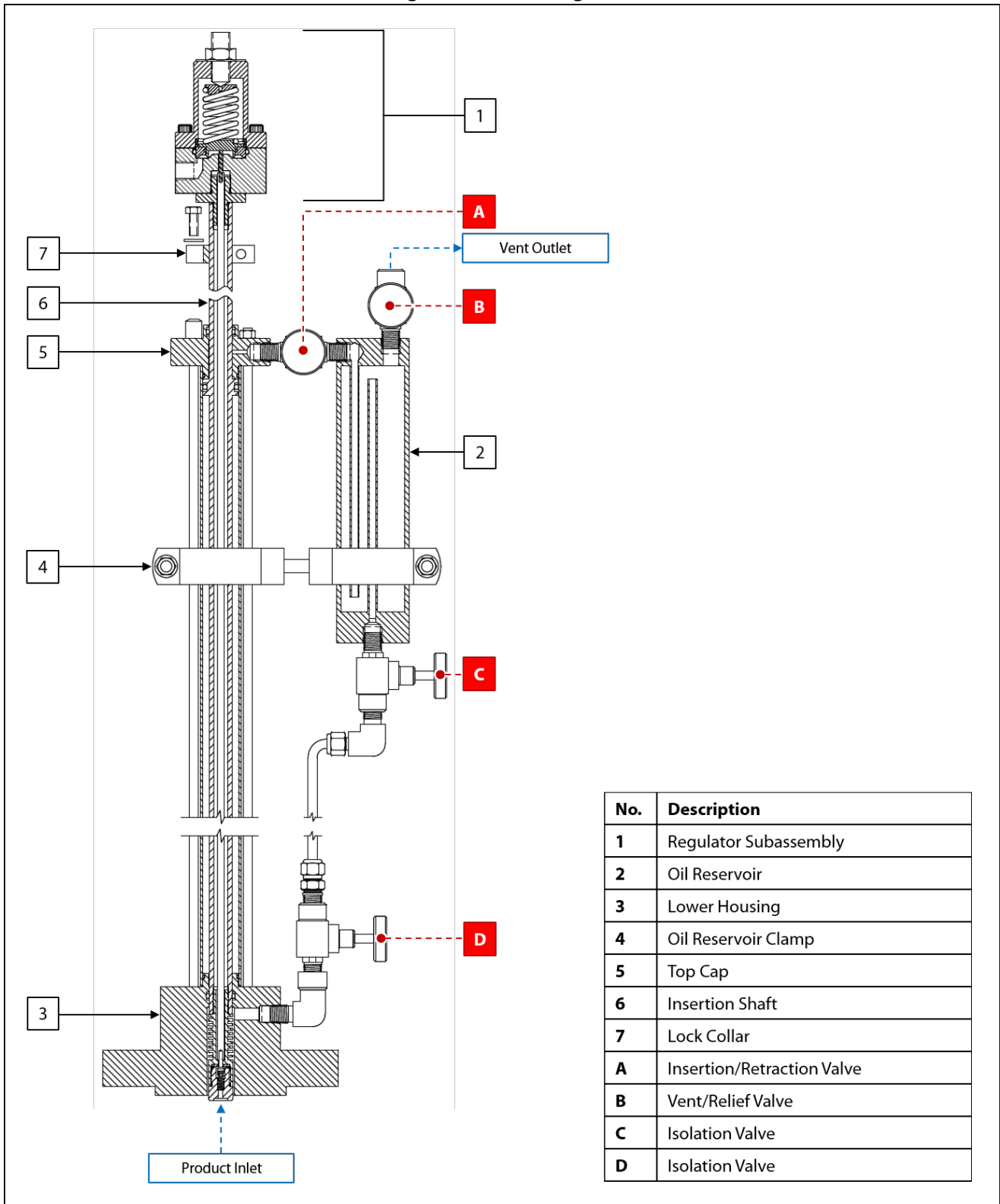
Figure 1: IRA-24 Diagram
