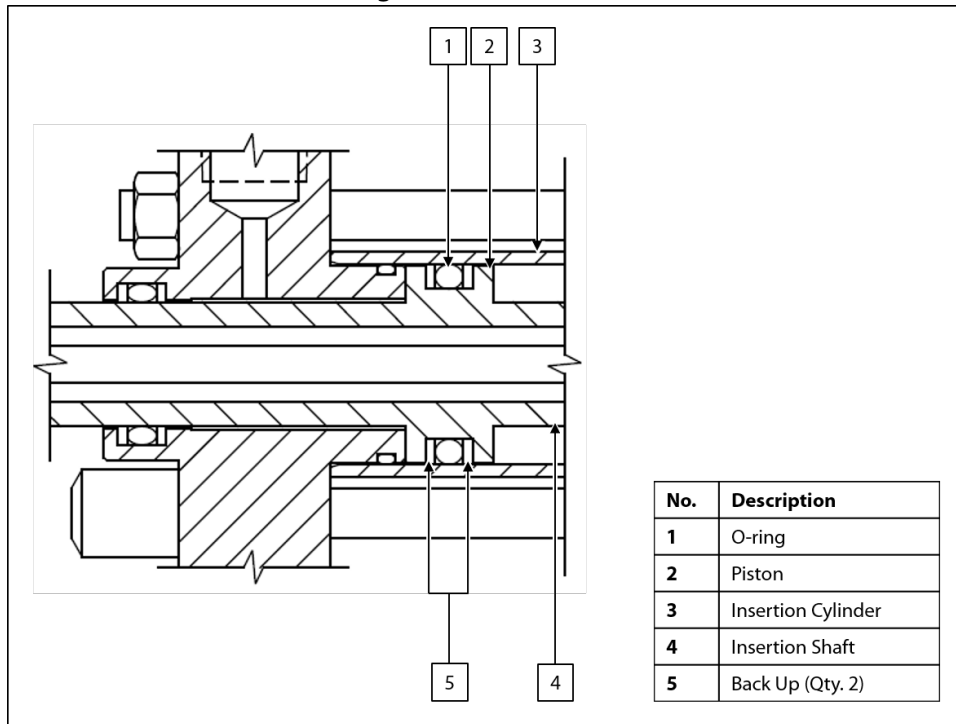
Figure 13: Shaft Detail
