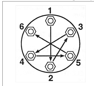
Figure 14: Cross-Bolting Sequence
