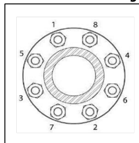
Figure 10: 8-Bolt Cross-Bolting Sequence
