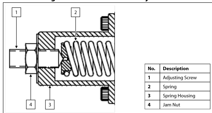
Figure 5: Outlet Pressure Adjustment
