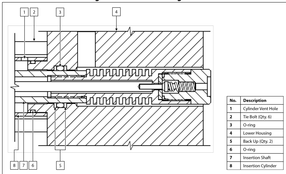
Figure 12: Lower Housing Detail
