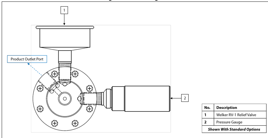
Figure 2: Port Diagram
