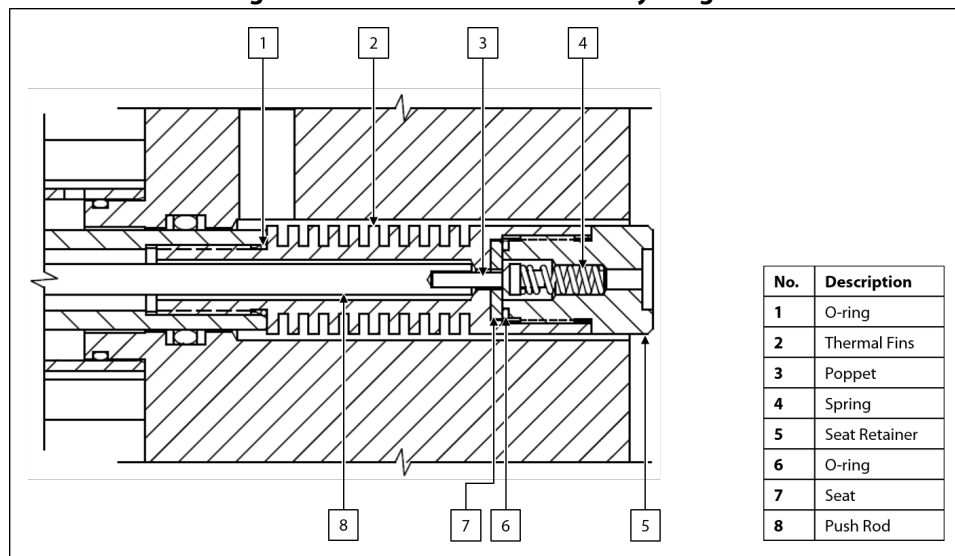
Figure 7: Thermal Fin Subassembly Diagram
