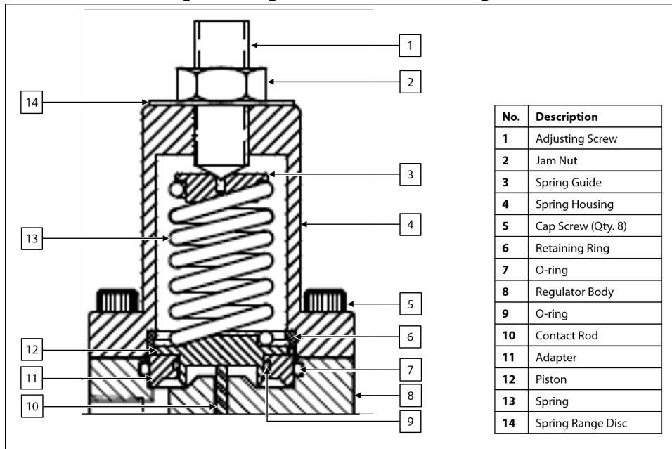
Figure 9: Regulator Maintenance Diagram
