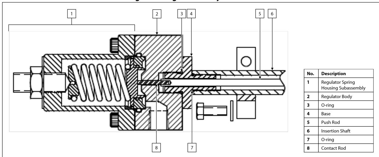
Figure 8: Regulator Body and Base
