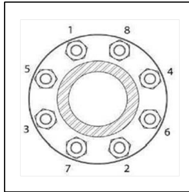
Figure 3: Cross-Bolting Sequence
