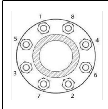
Figure B3: Cross-Bolting Sequence
