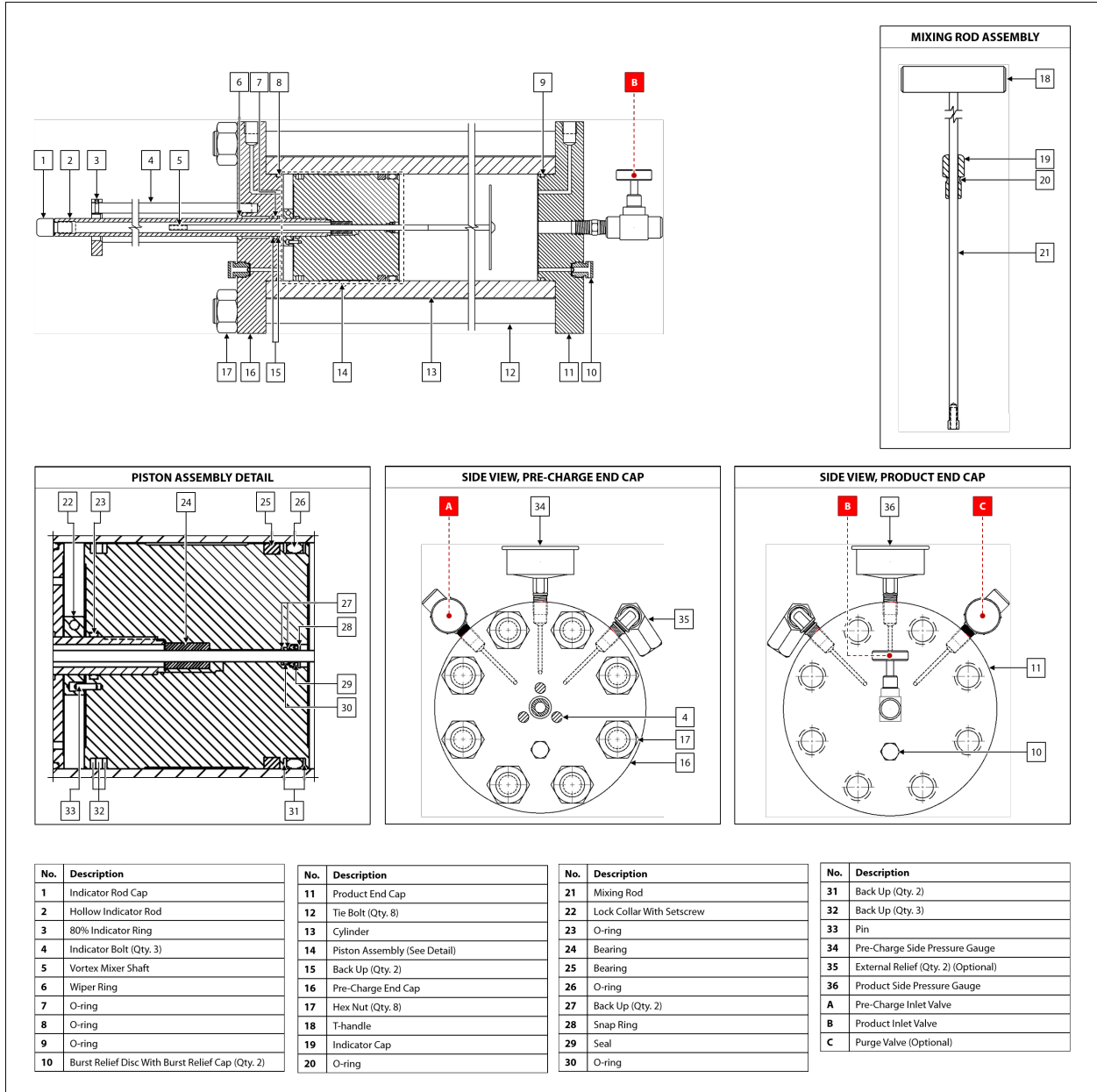
Figure B2: CP-80 With Vortex Mixer Maintenance Diagram
