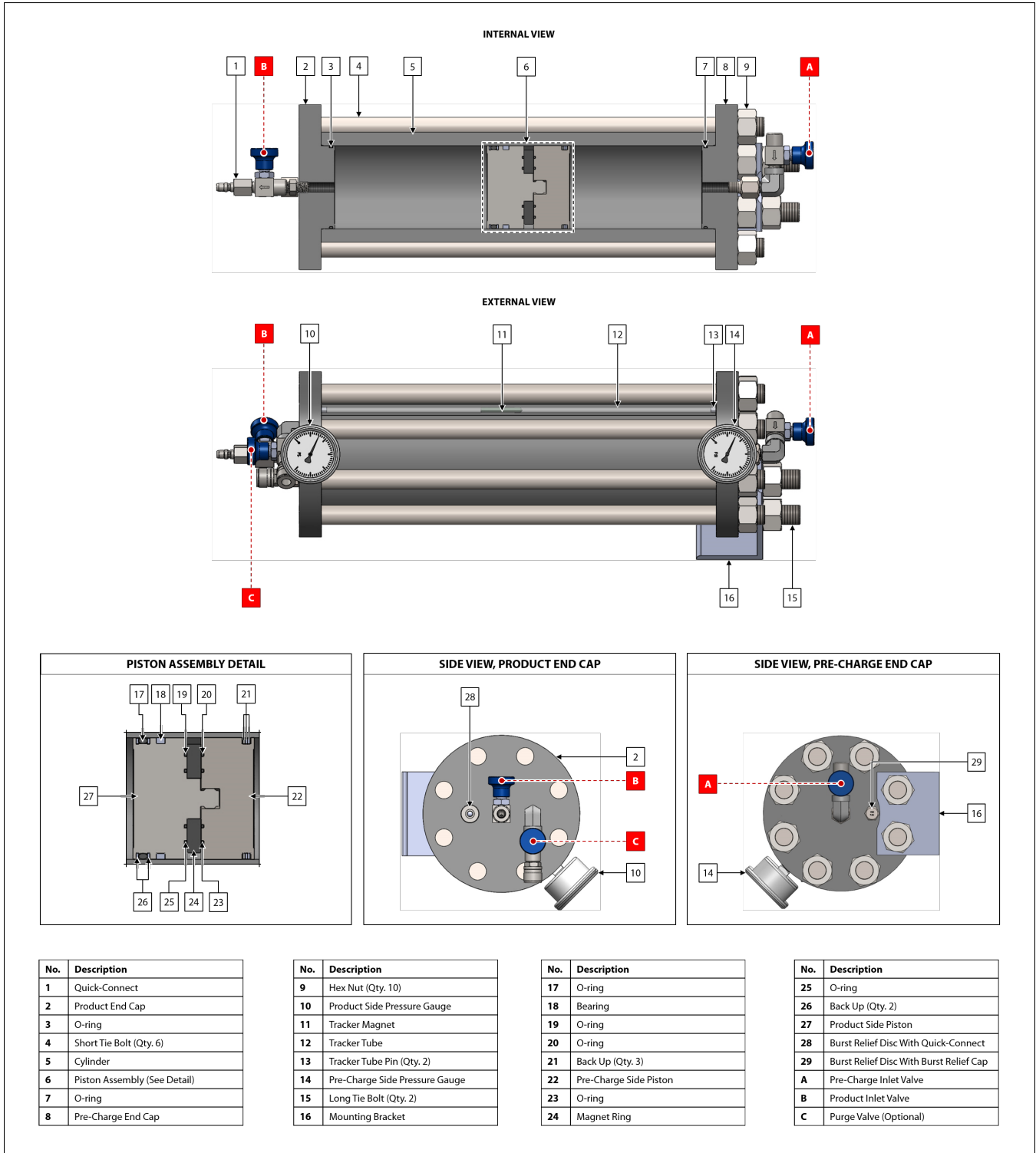
Figure 2: Standard CP-80 Maintenance Diagram
