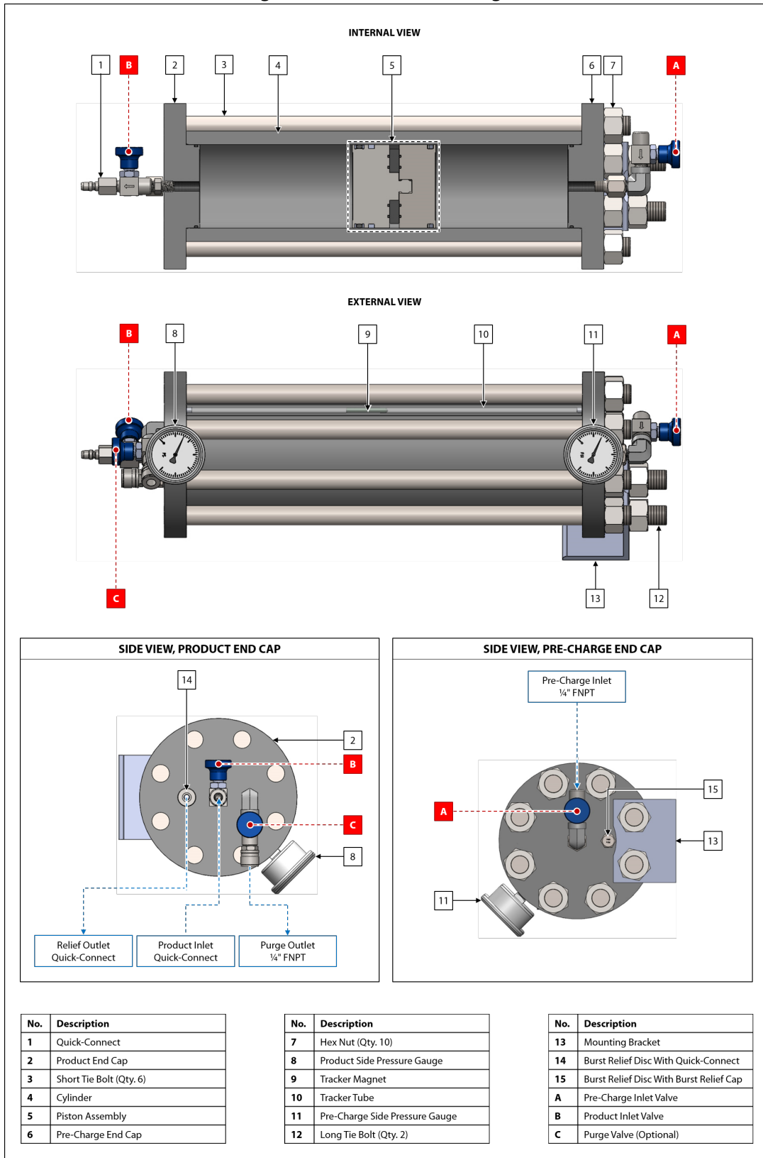
Figure 1: Standard CP-80 Diagram
