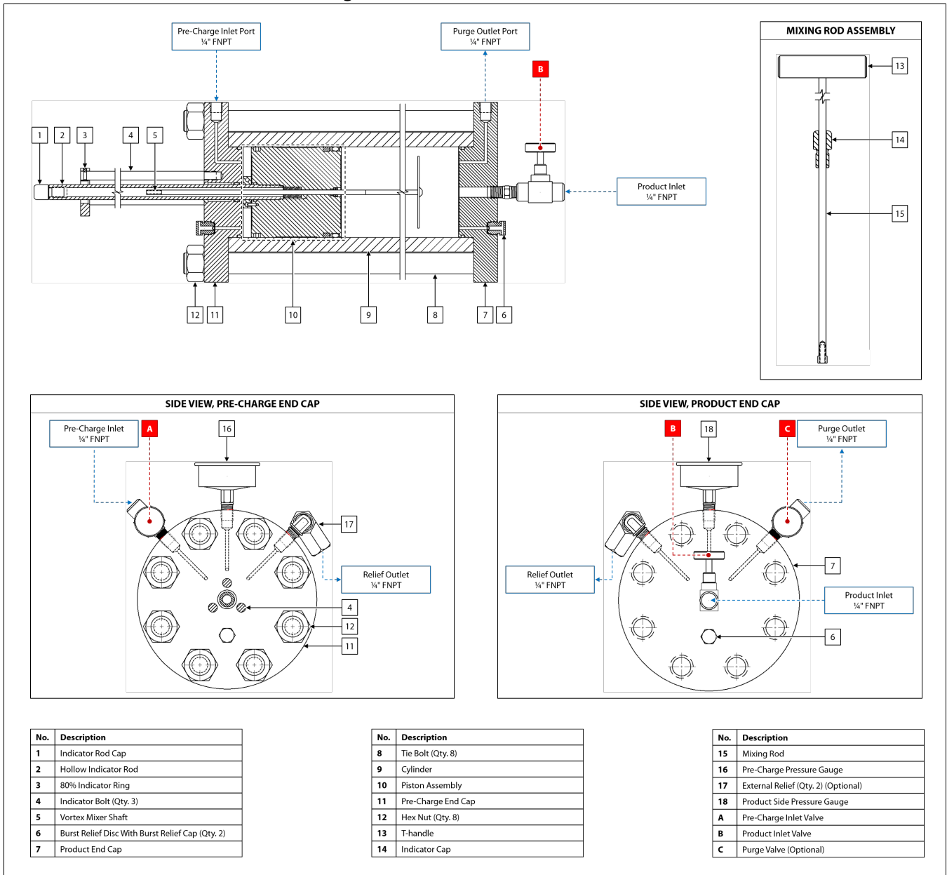
Figure B1: CP-80 With Vortex Mixer
