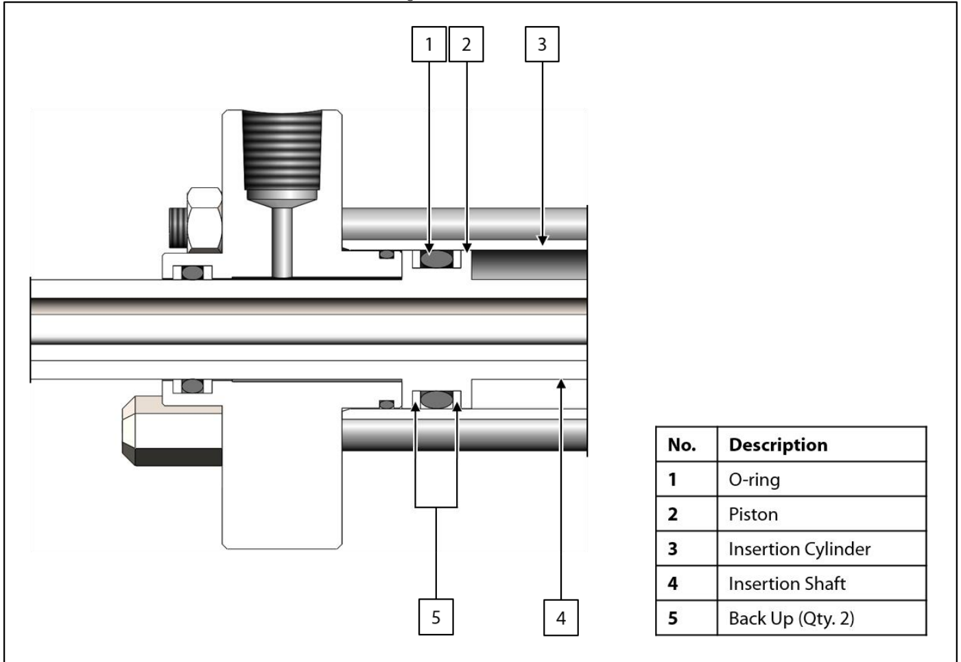
Figure 13: Shaft Detail
