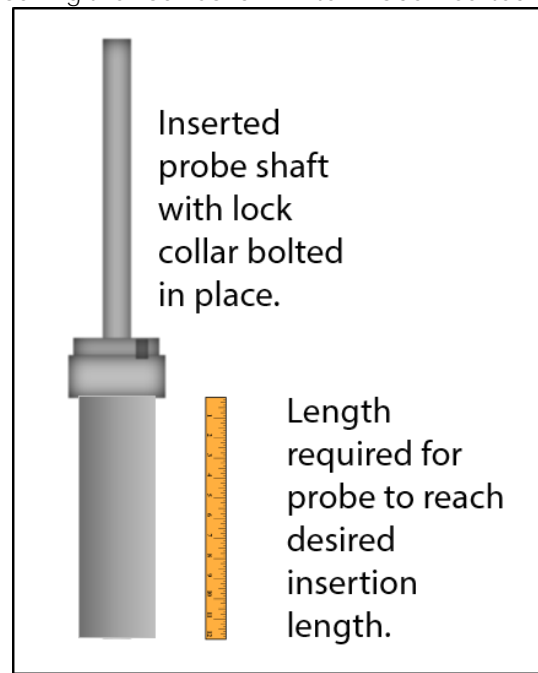
Figure 7: Locking the Lock Collar – After Probe Inserted Into Pipeline
