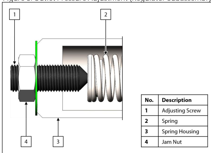
Figure 6: Outlet Pressure Adjustment (Regulator Subassembly)
