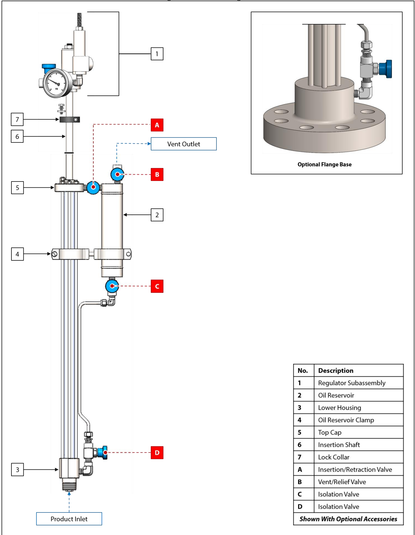
Figure 1: IRA-4SS Diagram
