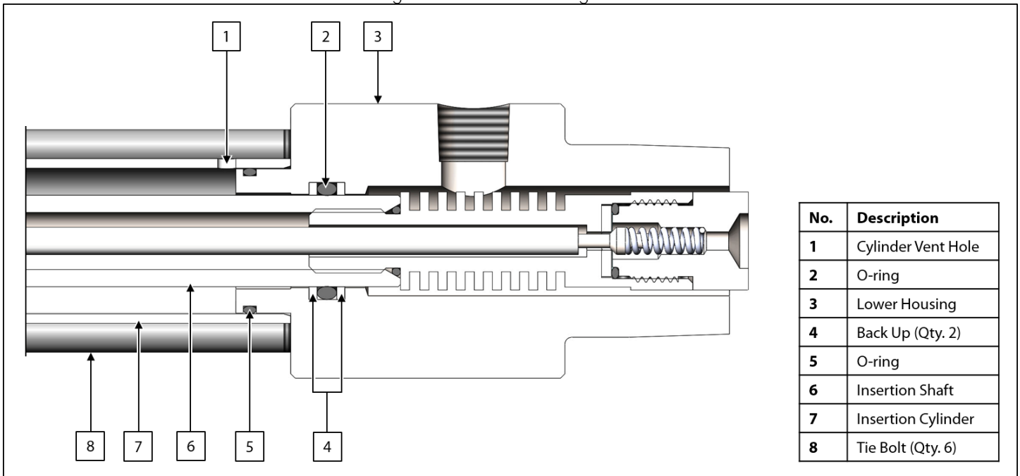
Figure 12: Lower Housing Detail
