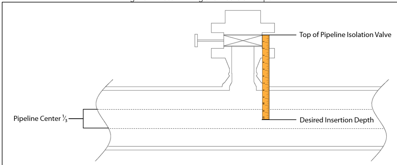
Figure 4: Determining the Insertion Depth
