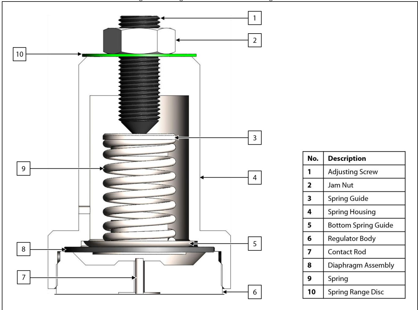
Figure 10: Regulator Maintenance Diagram
