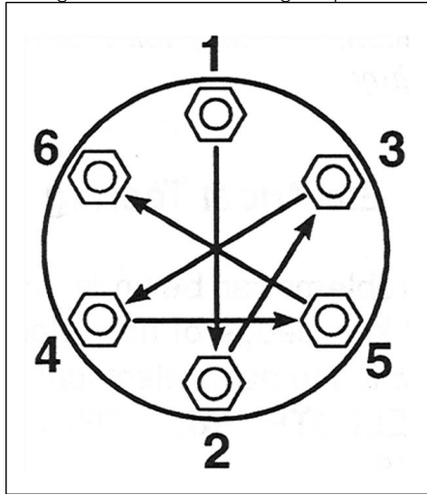
Figure 14: Cross-Bolting Sequence
