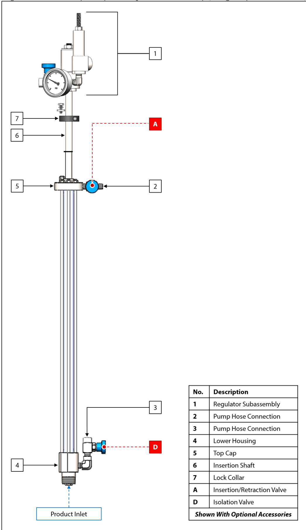
Figure 2: IRA-4SS Setup for Optional Hydraulic Hand Pump (Flanged Option Not Shown)
