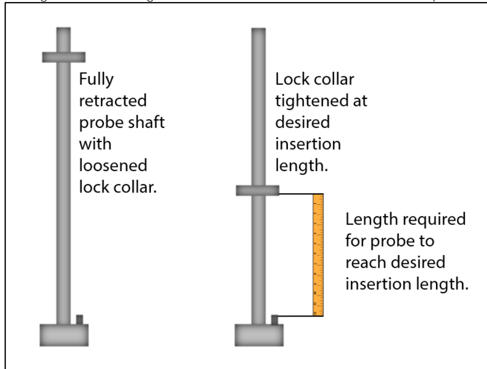
Figure 5: Positioning the Lock Collar – Before Probe Inserted Into Pipeline
