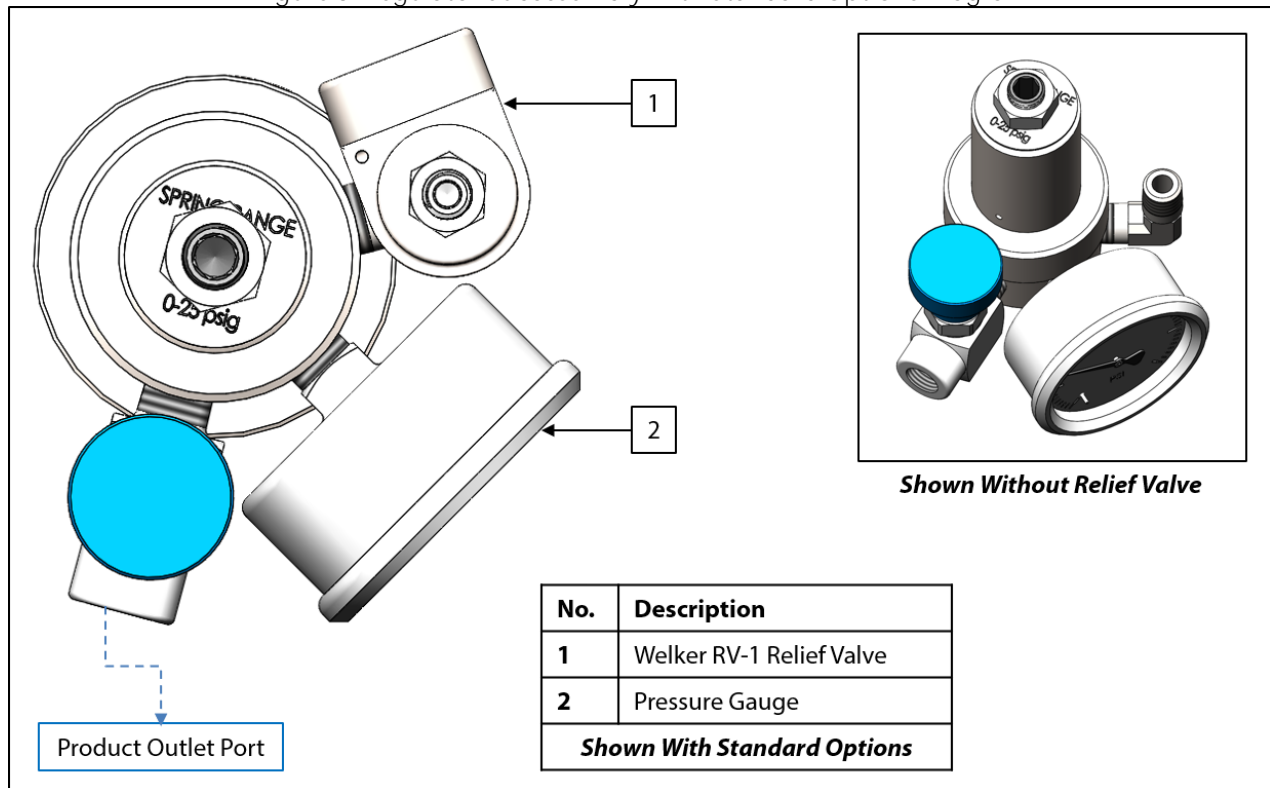
Figure 3: Regulator Subassembly With Standard Options Diagram
