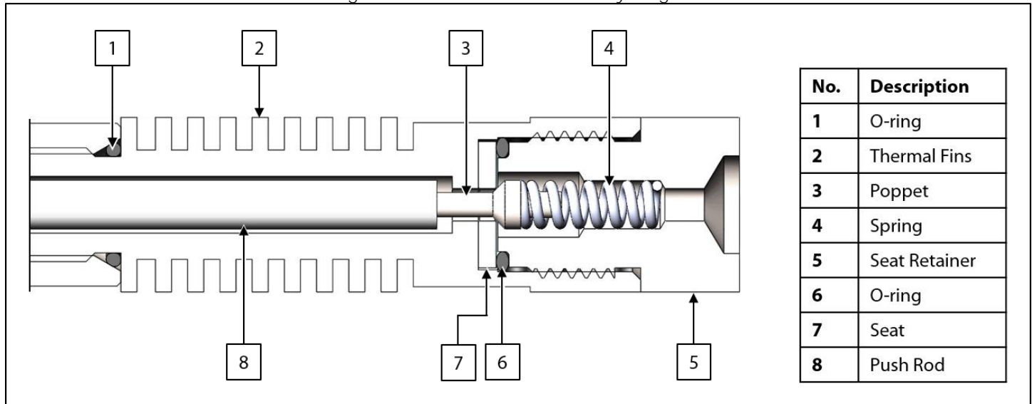
Figure 8: Thermal Fin Subassembly Diagram
