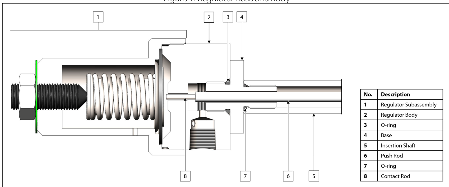
Figure 9: Regulator Base and Body
