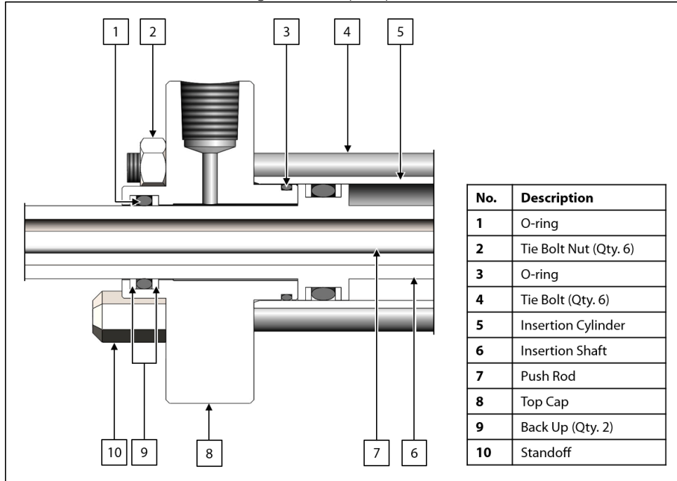
Figure 11: Top Cap Detail
