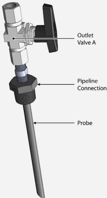
Welker® SP-5 Sample Probe
