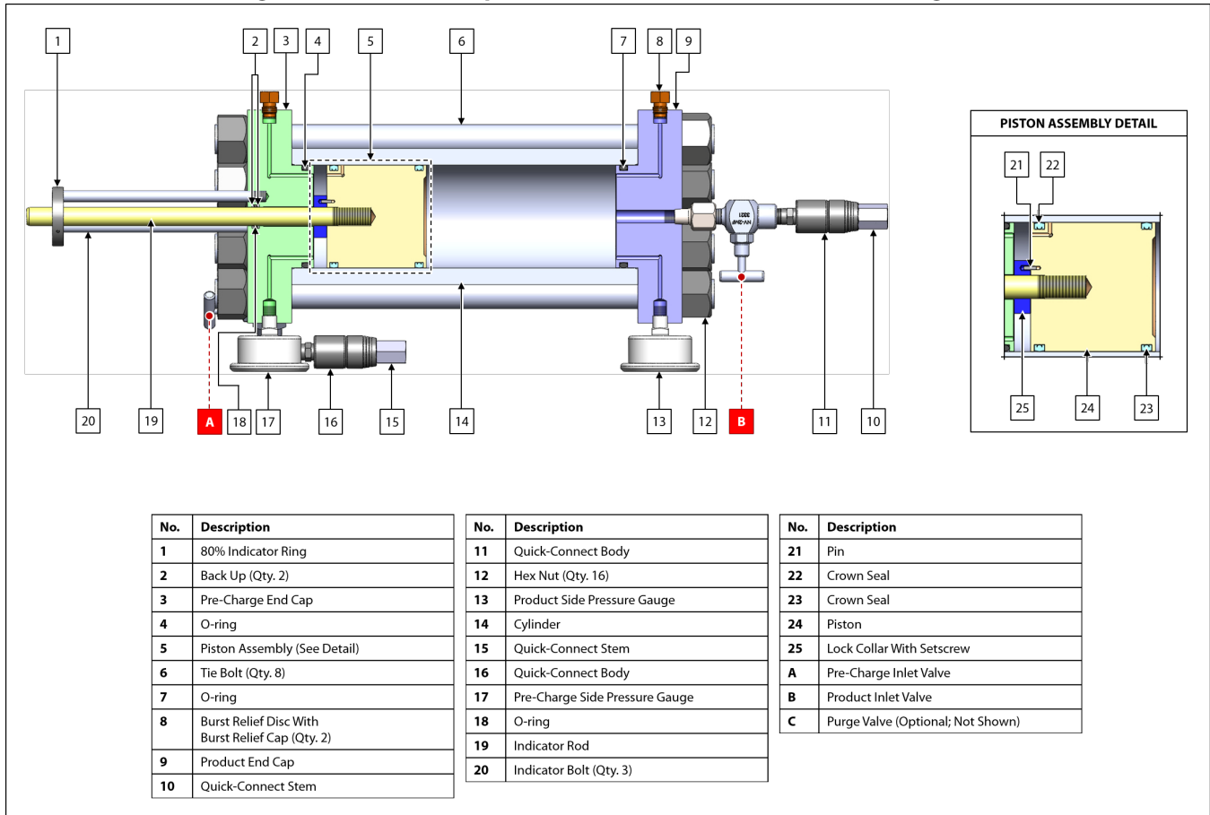
Figure 4: CP-11 With Optional Quick-Connects Maintenance Diagram
