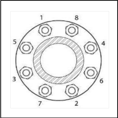
Figure 5: Cross-Bolting Sequence
