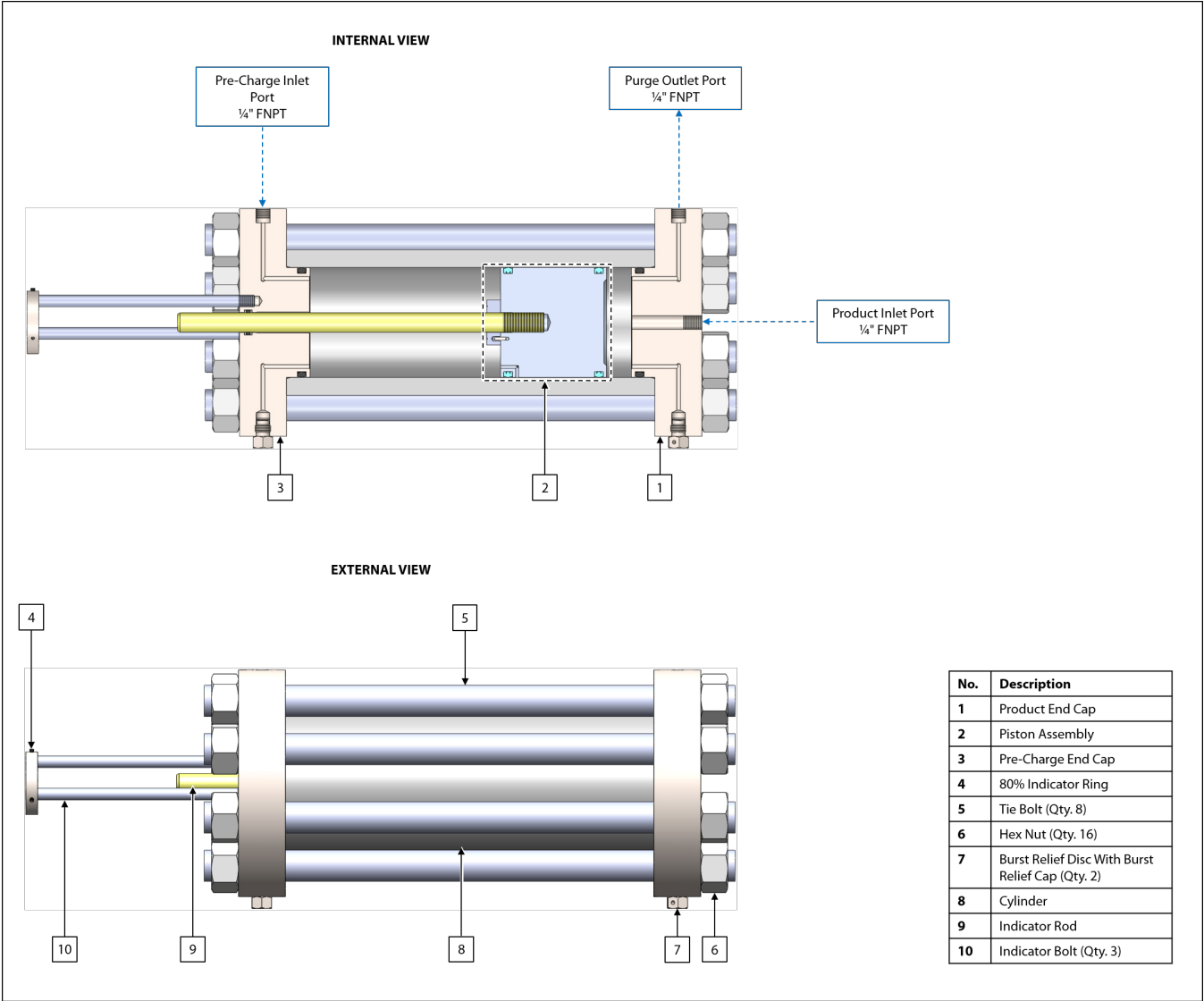
Figure 1: Standard CP-11 Diagram
