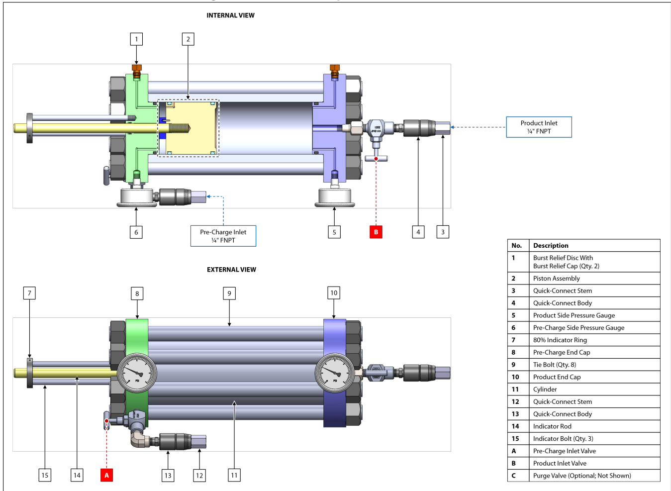
Figure 2: CP-11 With Optional Quick-Connects
