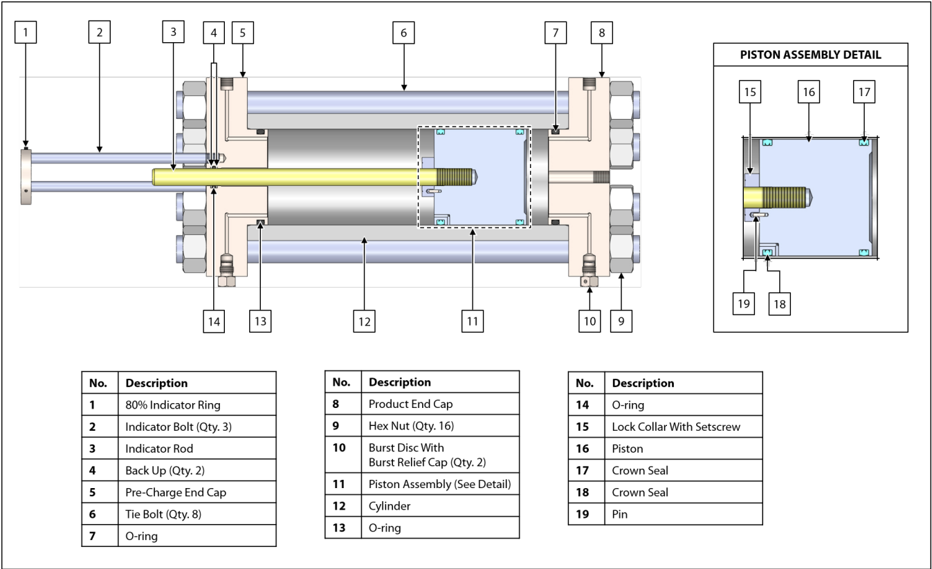
Figure 3: CP-11 Maintenance Diagram
