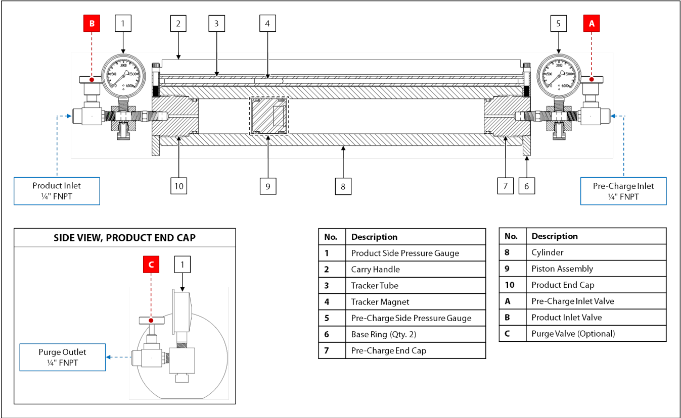
Figure 1: Standard CP-81 Diagram
