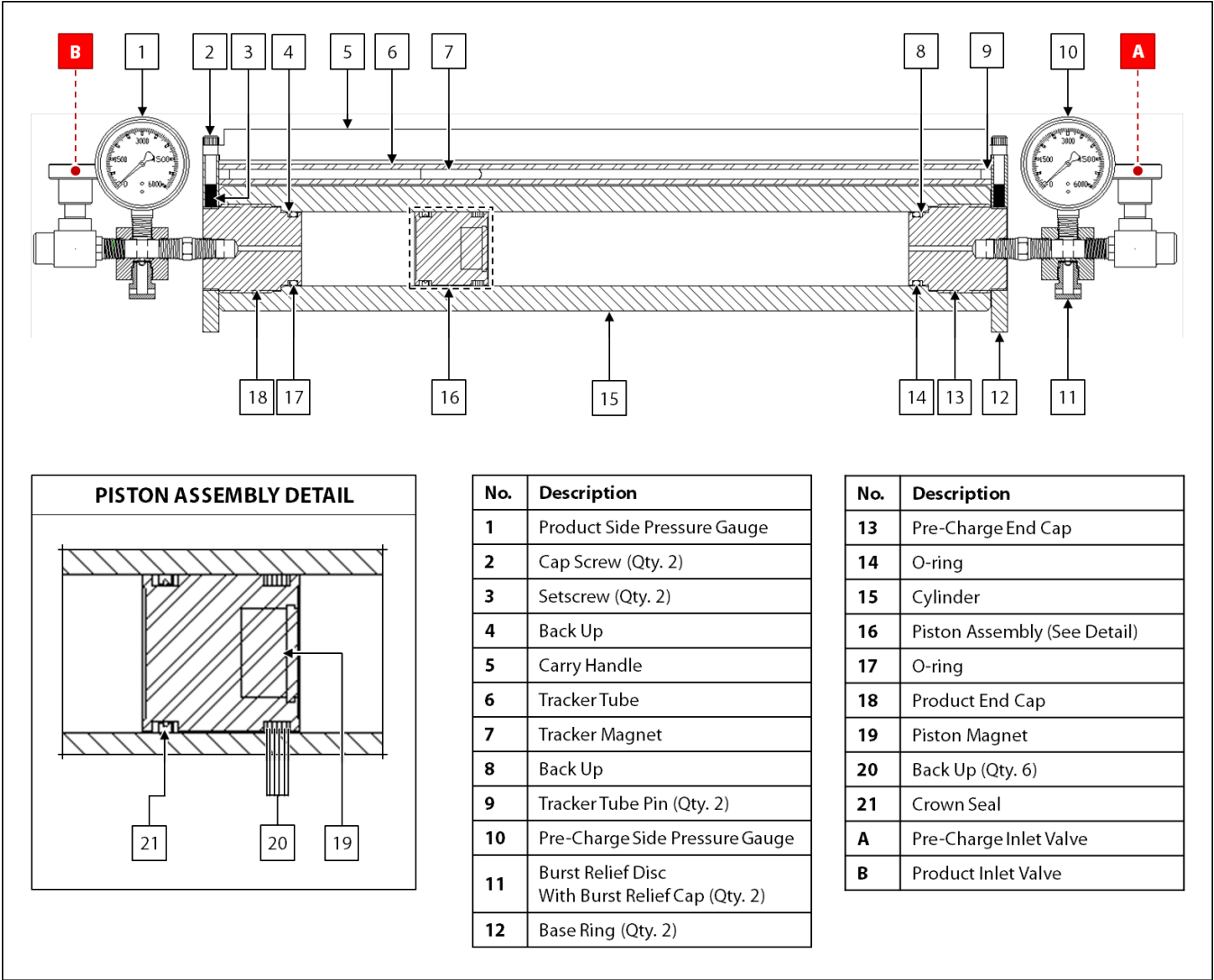
Figure 2: Standard CP-81 Maintenance Diagram
