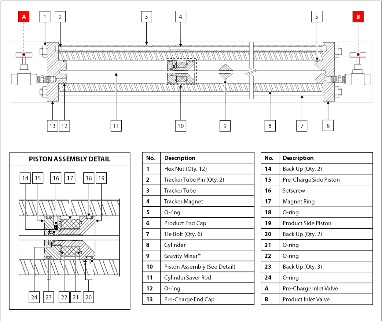
Figure B2: CP-81 With Gravity Mixer™ Maintenance Diagram
