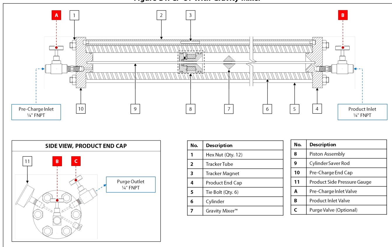
Figure B1: CP-81 With Gravity Mixer™
