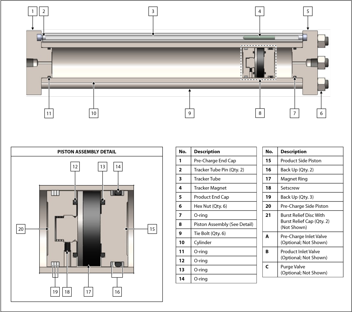
Figure 2: CP-24 Maintenance Diagram
