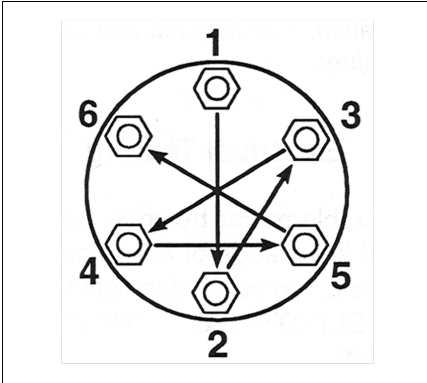
Figure B3: Cross-Bolting Sequence
