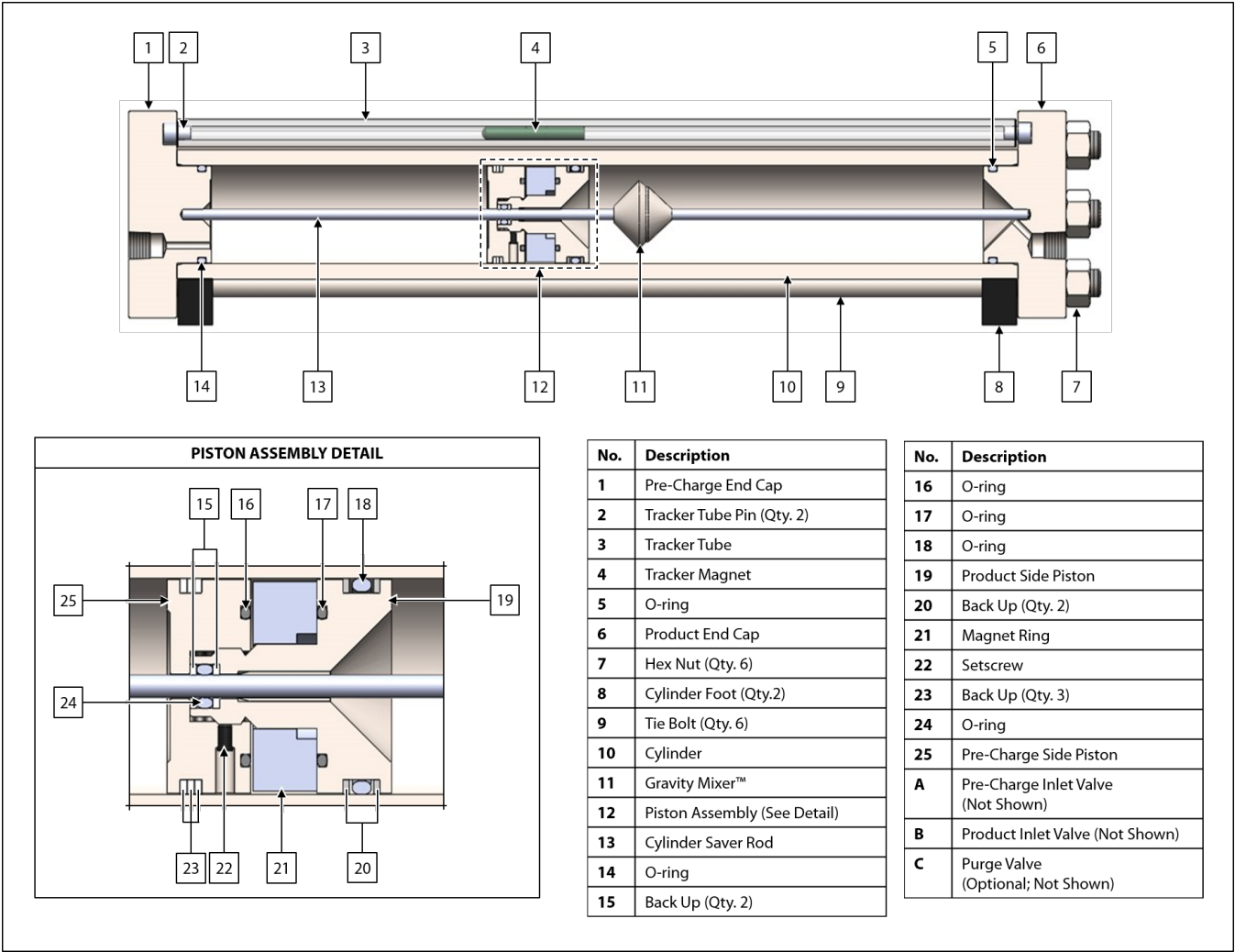
Figure B2: CP-24 With Gravity Mixer™ Maintenance Diagram
