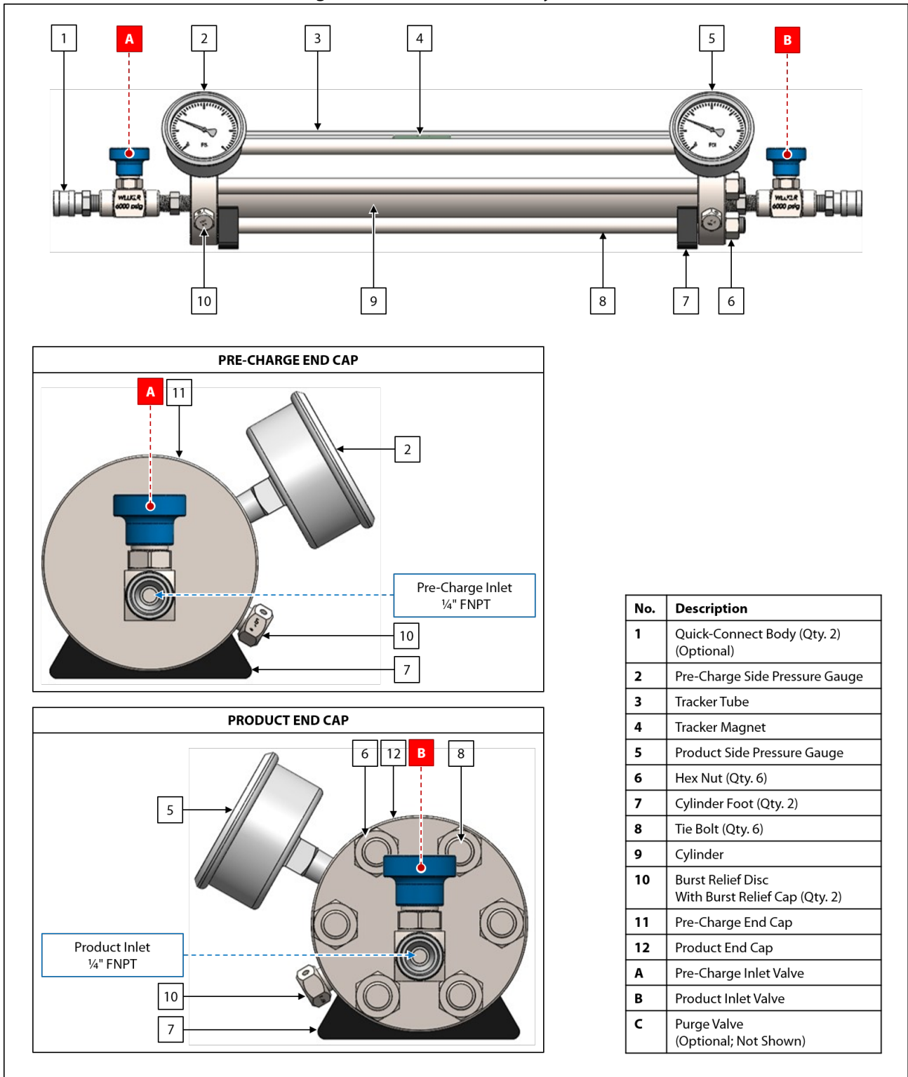
Figure B1: CP-24 With Gravity Mixer™
