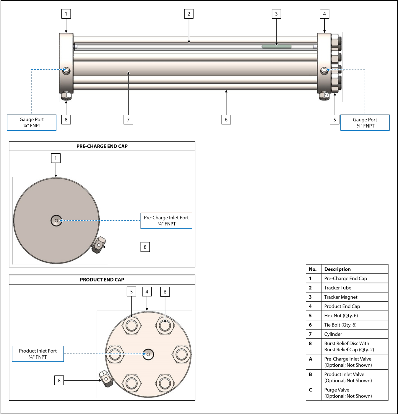
Figure 1: CP-24 With Magnetic Indicator
