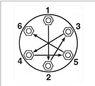
Figure 3: Cross-Bolting Sequence
